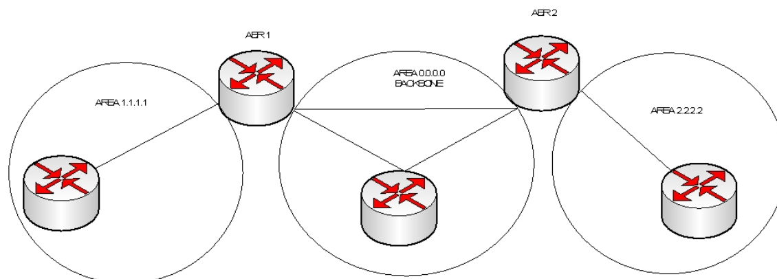
Fig. 1: Different areas in an OSPFv3 network.
